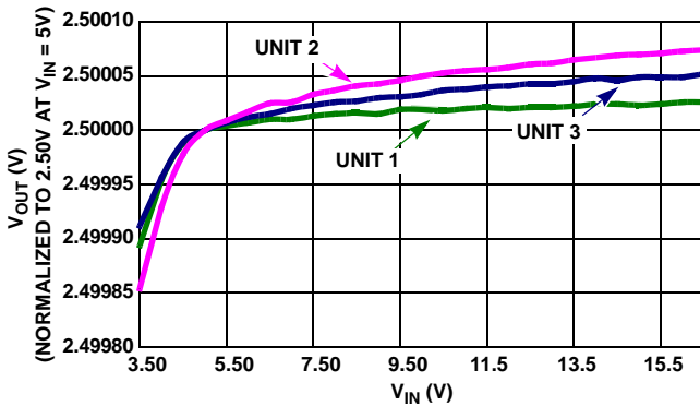
FIGURE 4. LINE REGULATION
