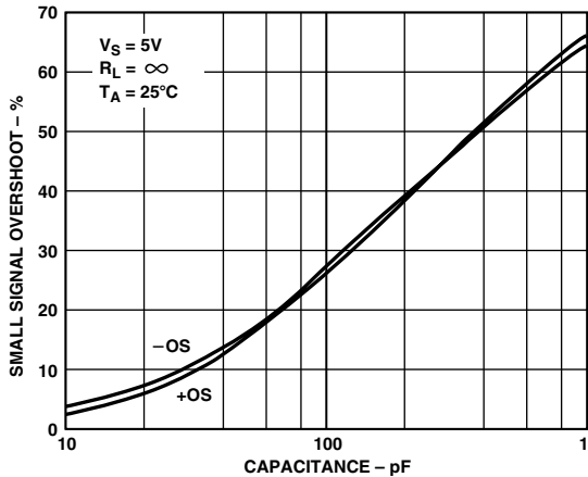
TPC 30. Small Signal Overshoot vs. Load Capacitance
