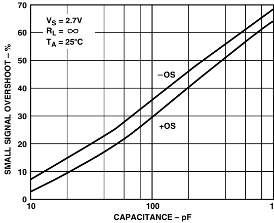
TPC 29. Small Signal Overshoot vs. Load Capacitance
